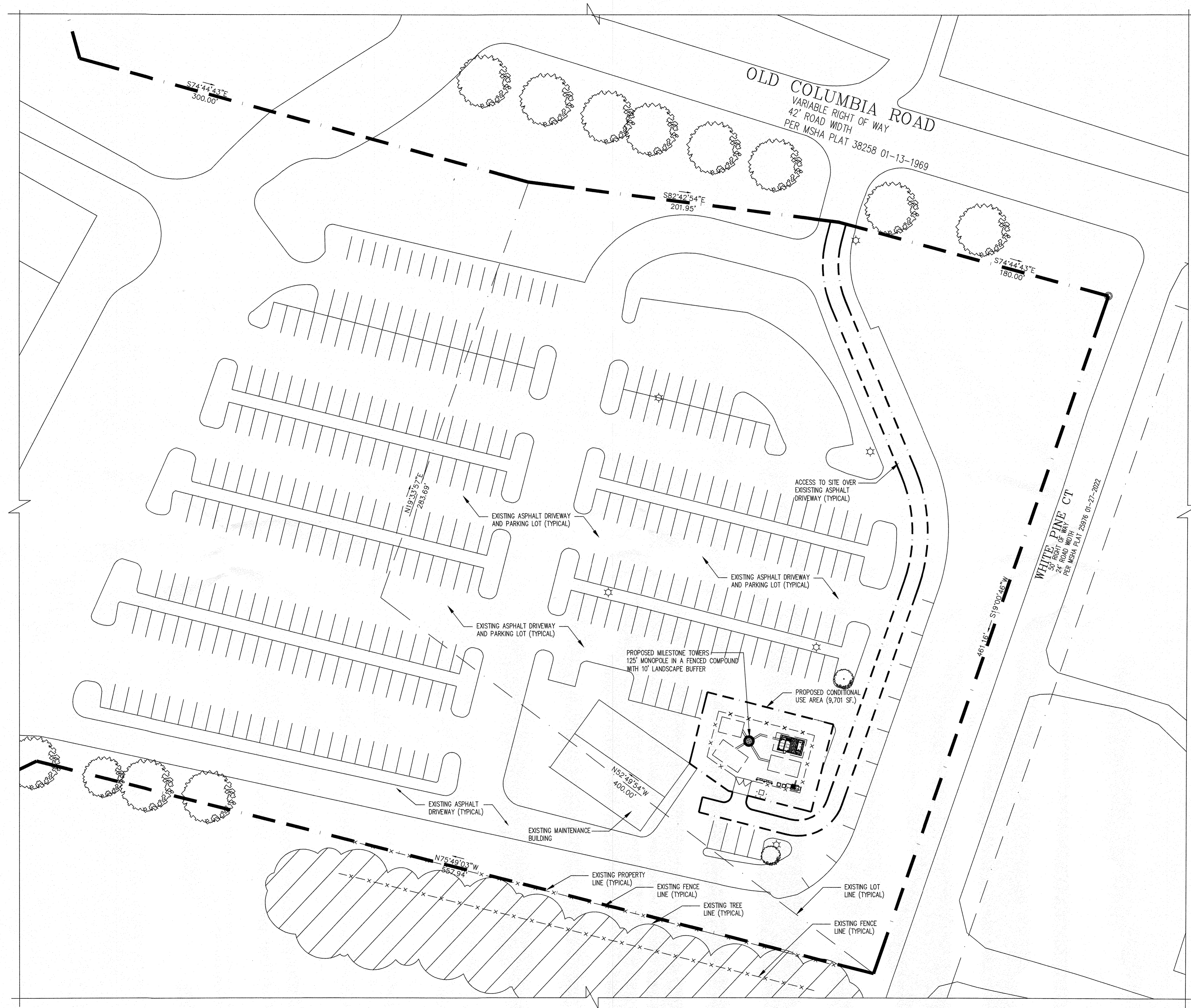
CONDITIONAL USE PLAN SCALE: 1" = 30'
