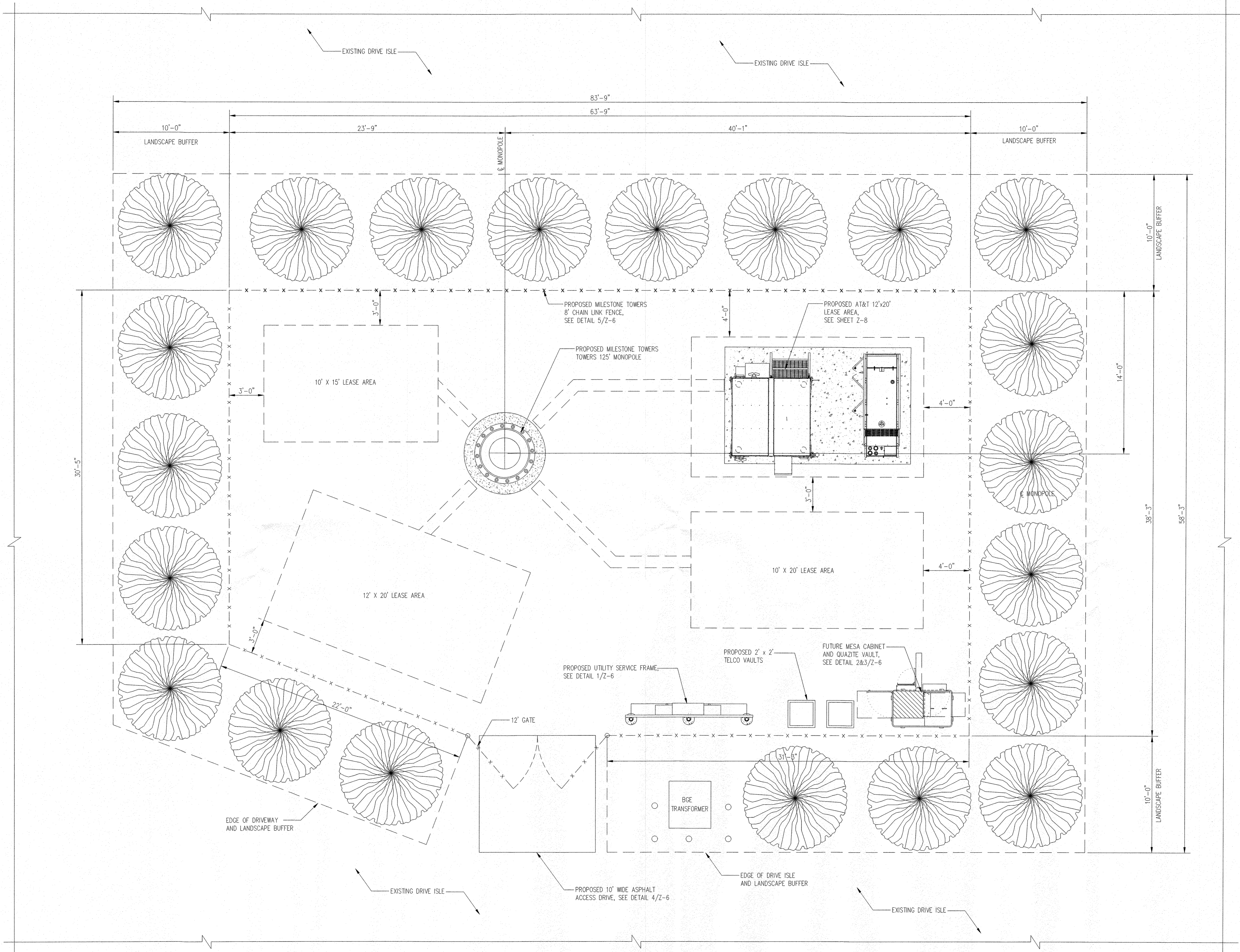
COMPOUND PLAN SCALE: 1/4" = 1'-0" 1 Z-4 TRUE NORTH
