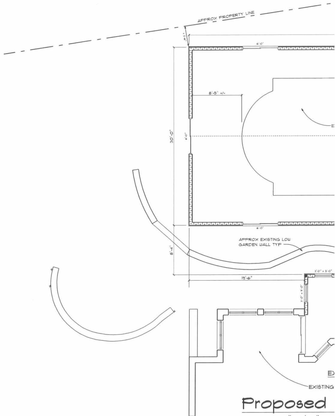
Cadigan Pool Enclosure 1/2/2025 Schematic
